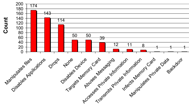
Figure 2: Smartphone malware effects
