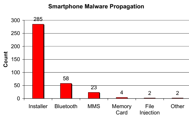
Figure 3: Malware propagation
