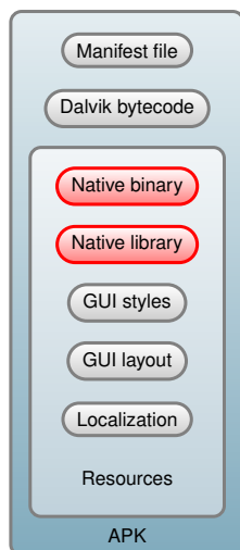
Figure 5: The Android Installation file containing malicious components
