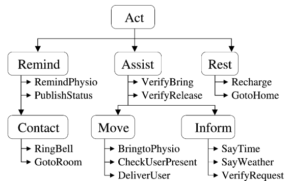
Fig. 4. Dialog problem action hierarchy.
