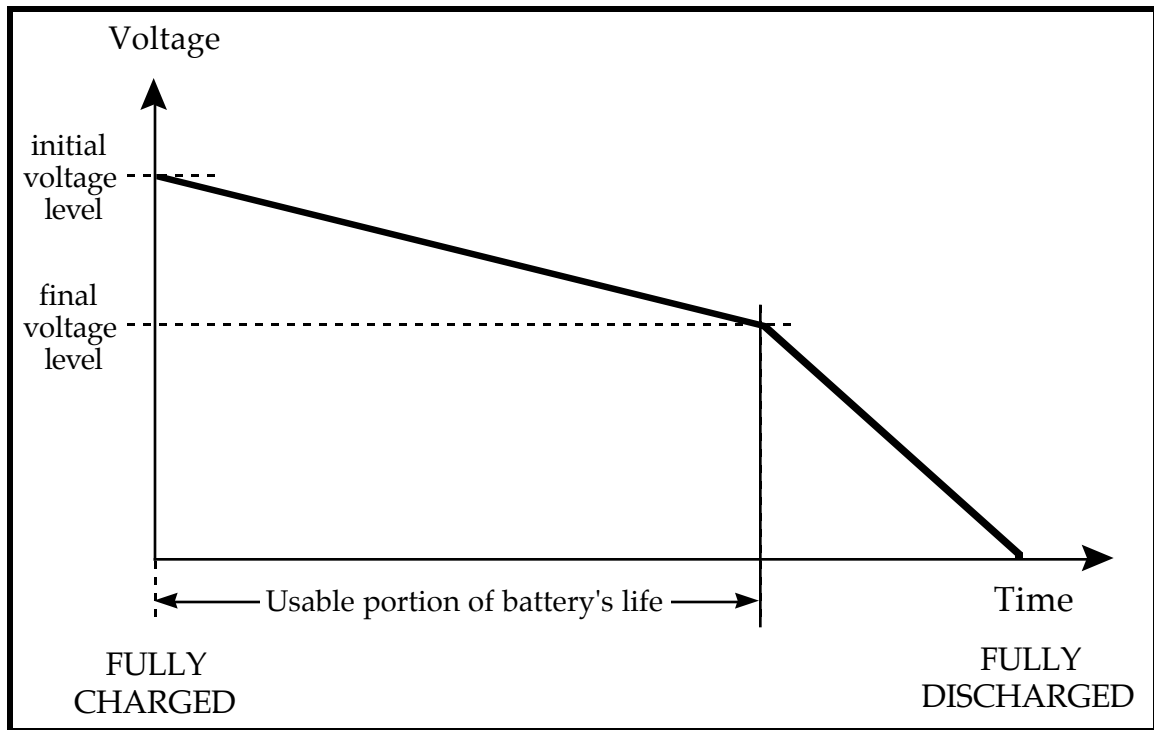
FIGURE 3. Idealized lead-acid cell discharge curve.
