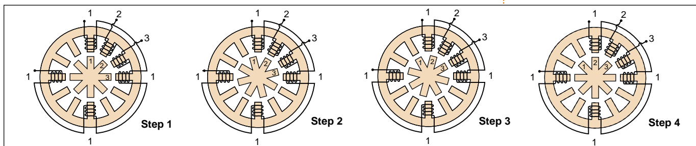
Figure 22 — In a variable reluctance motor, the multi-tooth armature provides higher holding torque at each 15° rotary step. Motion is accomplished through coordinated energizing of the stator poles from step 1 through 4.
