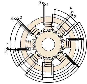
Figure 23 — Hybrid synchronous stepping motors gain superior performance by combining the best of permanent magnet and variable reluctance stepping motors.
