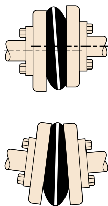
Figure 19 — Shaft couplings adjust for and accommodate angular and parallel misalignment between rotating shafts.
