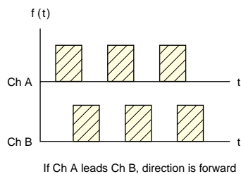
Figure 30 — Quadrature encoder output provides direction as well as position feedback.
