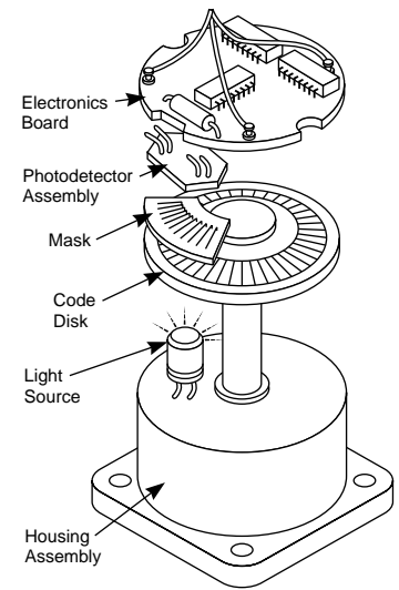
Figure 27 — Optical rotary encoders commonly use a stationary mask between the code wheel and the detector.
