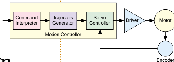
Figure 33 — Functional block diagram of controller operations.
