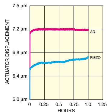
Figure 25 — Comparing actuator creep—electrostrictive actuators are superior to conventional PZTs when trying to maintain position over time. The figure shows the results after one hour with a voltage step applied at time-zero.
