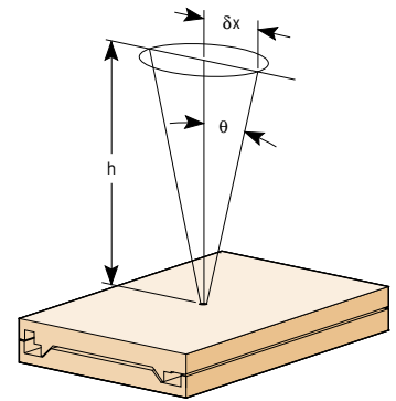
Figure 8 — Abbe error can be reduced by minimizing the height, h , from the stage surface.
