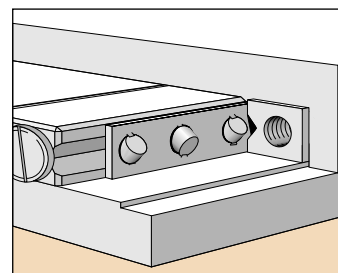
Figure 15 — Crossed-roller bearings have all the advantages of ball bearings with greater stiffness and load capacity.
