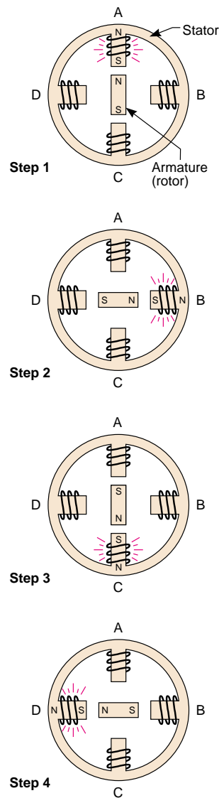
Figure 21 — Rotation in a stepper motor is generated by alternately energizing and de-energizing the poles in the motor's stator creating torque which turns the rotor.
