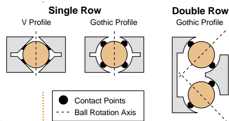
Figure 14 — The type of bearing way, ball diameter and number of balls affect the load capacity of a stage.
