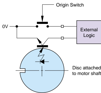
Figure 29 — To get submicron repeatability using an index pulse from an encoder, homing should always be approached from the same direction.
