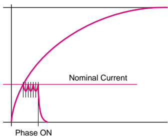
Figure 37 — A high voltage chopper helps a stepper motor reach full current faster enabling higher speeds.
