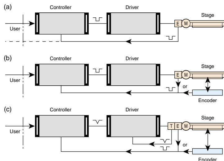
Figure 31 — Closed-loop systems. a) Using indirect metrology rotary encoder b) Using direct metrology linear encoder c) Using encoder for position feedback and tachometer for velocity control.
