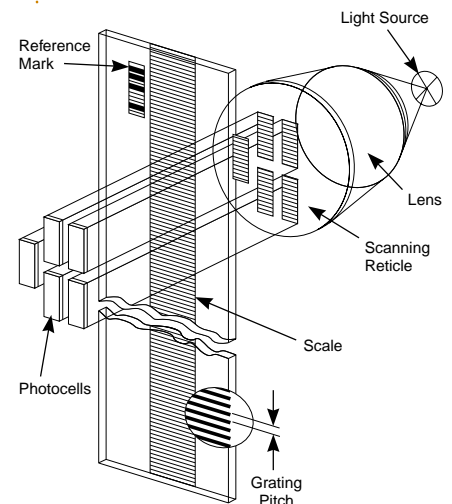
Figure 28 — Optical linear encoders direct light through a glass scale with an accurately etched grating to photocells on the opposite side.
