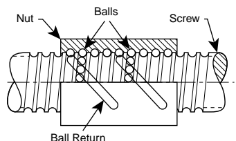
Figure 17 — Ball screws use recirculating balls to reduce friction and gain higher efficiency than conventional lead screws.
