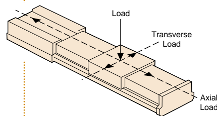
Figure 10 — Load capacity specifications refer to loads which are centered and perpendicular.
