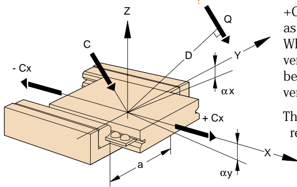
Figure 11 — Selecting the proper stage requires an understanding of how loads are applied.
