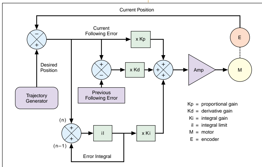
Figure 41 — PID control implemented using position feedback.
