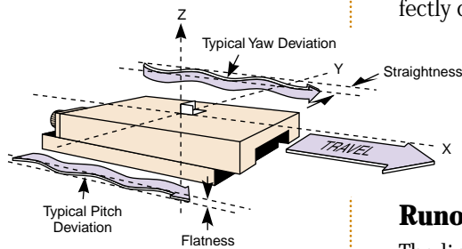
Figure 6 — Off-axis errors in a linear stage.
