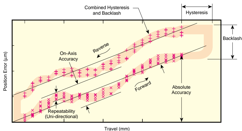
Figure 2 — Error vs. position for a stage translated four times in each direction. This figure shows graphically the difference between backlash and hysteresis.
