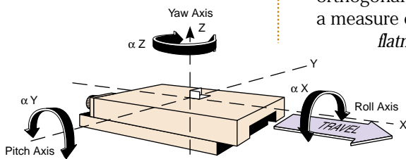
Figure 7 — Roll, pitch, and yaw are defined with respect to the direction of travel.
