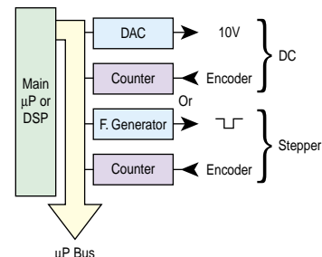
Figure 34 — With centralized motion processing, all axes are controlled by a single microprocessor.
