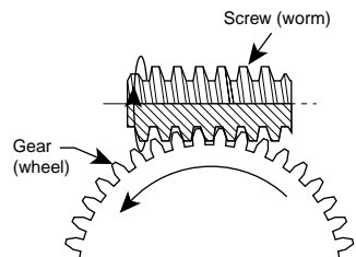
Figure 18 — Worm drive systems can provide high speed and high torque.
