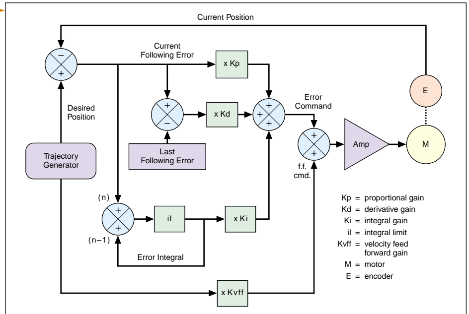
Figure 42 — Adding a feed forward loop to the PID controller reduces following error and improves overall system performance.
