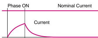
Figure 36 — Exponential current build-up in the motor is too slow for high speed applications.
