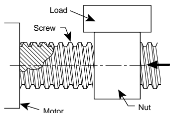
Figure 16 — As the lead screw rotates, the load is translated in the axial direction of the screw.
