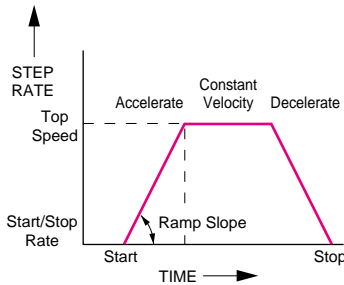
Figure 40 — Trapezoidal motion profiles are required to obtain higher speeds without skipping steps or stalling.
