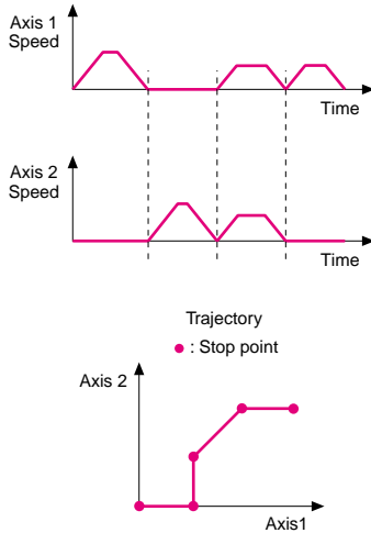
Figure 43 — With synchronized motion, multiple axes may or may not move together.
