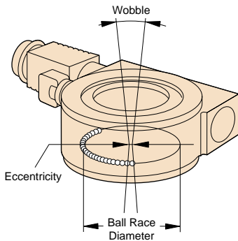
Figure 5 — Off-axis errors in a rotary stage.
