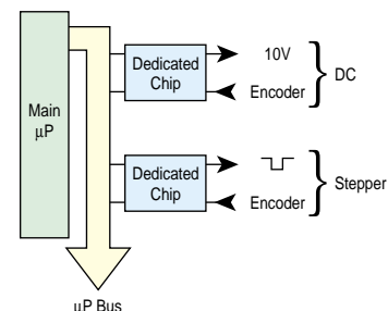
Figure 35 — Distributed motion processing provides dedicated motion controller chips for each axis coordinated by a central CPU.
