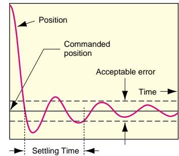
Figure 38 – How settling time is defined.
