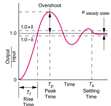
Figure 39 — Response for a system using only proportional control leads to overshoot and non-zero steady-state errors.
