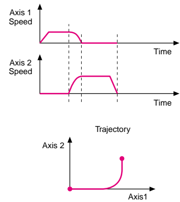
Figure 46 — Simple circular interpolation.
