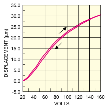
Figure 26 — Electrostrictive actuators have very little hysteresis.
