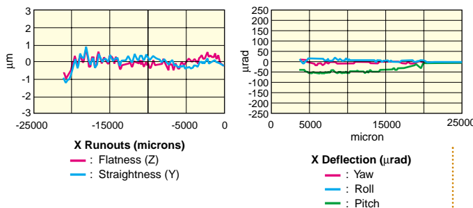
Figure 9 — Simplified schematic of Newport’s interferometric test setup for measuring off-axis errors and sample test results. High quality translation stages have sub-micron runout errors with angular deviations on the order of 100–150 µradians.
