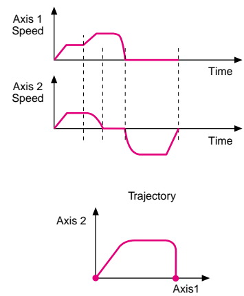
Figure 48 — Applications such as laser writing require unusual trajectories executed at constant speed.
